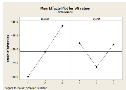
Fig 9: HC S/N Ratio Curve
