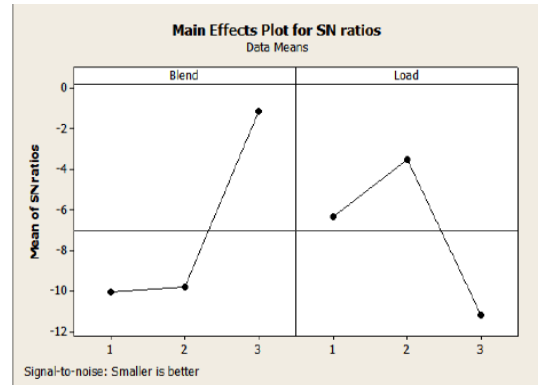
Fig 7: CO2 S/N Ratio Curve
