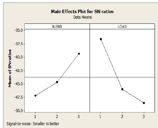
Fig 5: S/N Ratio NO Graph
