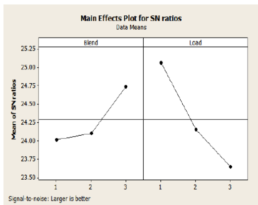
Fig 8: O 2 S/N Ratio Curve
