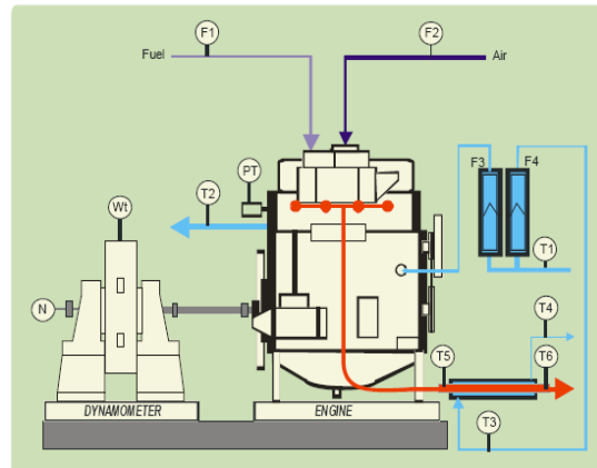
Fig 1: Line Diagram of Single Cylinder Four Stroke Diesel Engine
