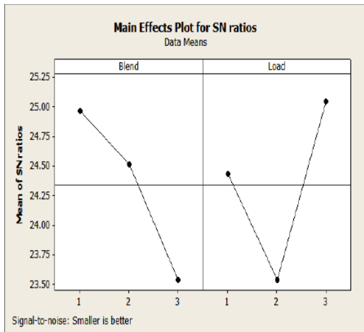
Fig 6: CO S/N Ratio Curve
