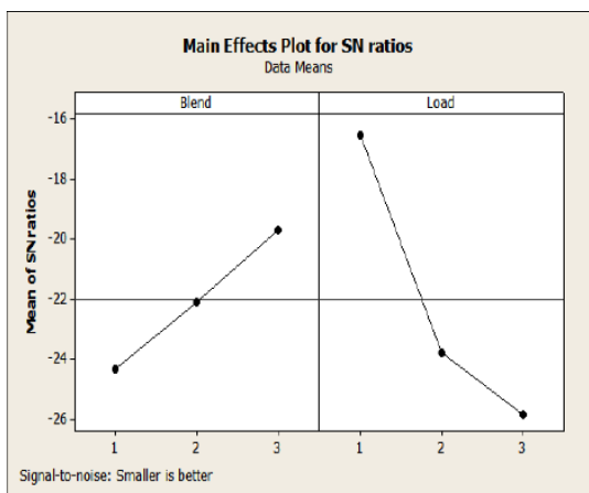
Fig 4: Opacity S/N Ratio Curve
